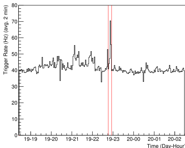
Fig. 12. On Dec 19 at approximately 10:46 PM, Notch 2 was de-activated for approximately 10 minutes. The vertical red lines enclose the duration of time during which Notch 2 was de-activated. A trigger rate above \sim 50 Hz incurs digitization deadtime. The spike in event rate shows that Notch 2 was crucial to keeping CW interference in check. Even with the LCP/RCP coincidence required by the ANITA-IV trigger, further mitigation of CW interference by the TUFF boards was necessary to avoid masking.
