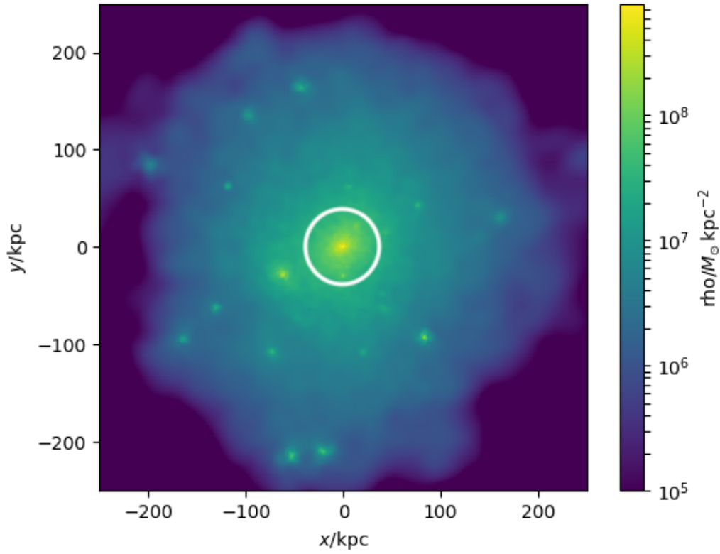
Figure 1: Projected map of stellar density in the stellar halo obtained with the implemented particle-tagging scheme. The method tracks all accretion and merger events in the history of a halo and paint stars at first infall based on a semi-analytical recipe. A white circle of radius 30 kpc highlights the typical size of the inner region of the halo, unresolved by this approach neglecting the effect of the central galaxy. This method is a key step towards generating dark matter halos with genetically modified merger histories and observing the resulting changes in stellar halo properties.
