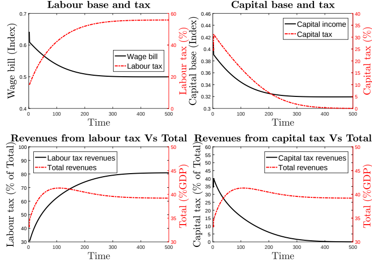
Figure 8: Optimal fiscal mix (CE=1.53%)
